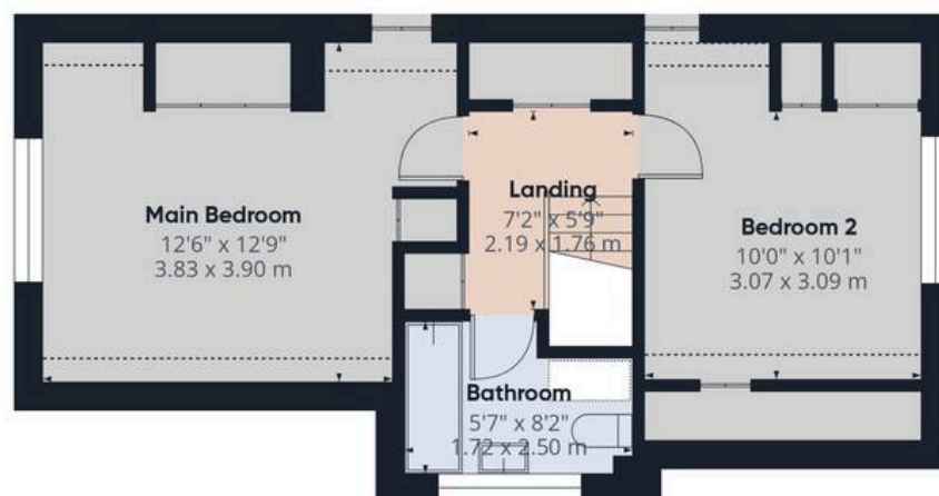
Floor 1 Building 1
